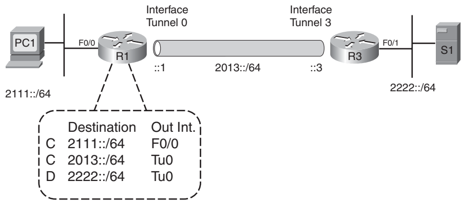
Key Topic Figure 18-3 IPv6 Point-to-Point Tunnel Concept
