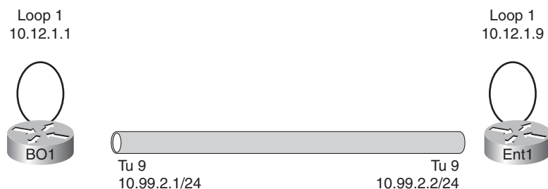
Figure 19-11 GRE Tunnel Topology and Addresses
