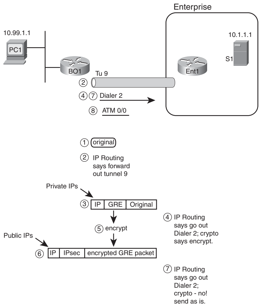
Figure 19-12 Example of Routing and Encapsulation with GRE over IPsec
