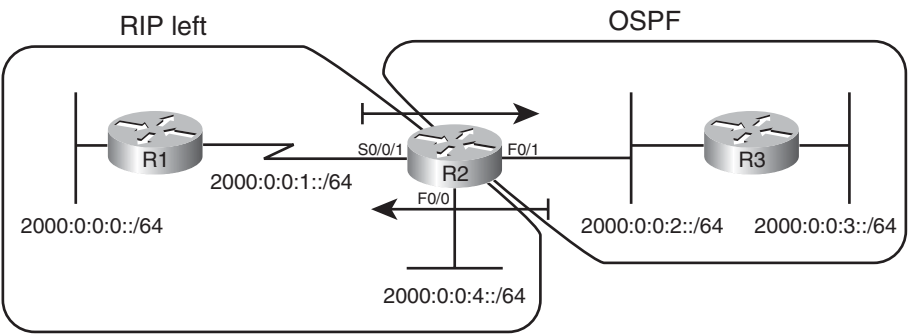
Figure 17-3 Redistribution Plan
