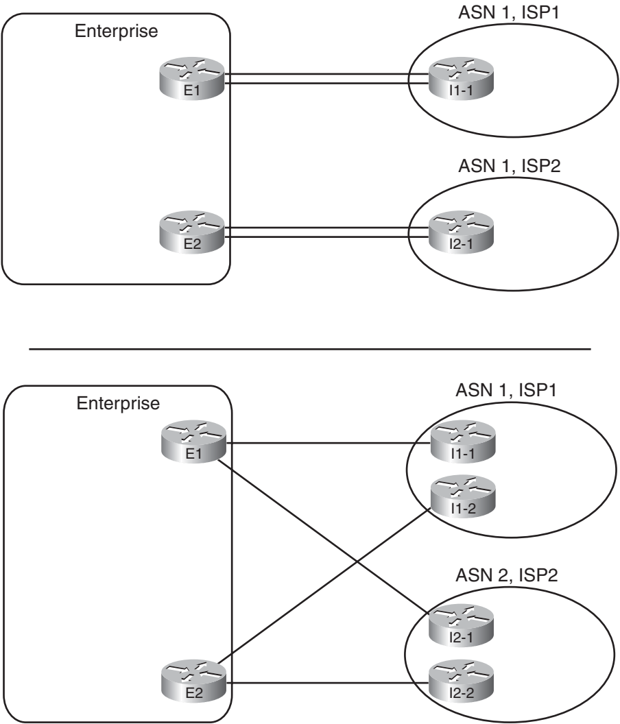
Figure 12-15 Dual-Multihomed Options
