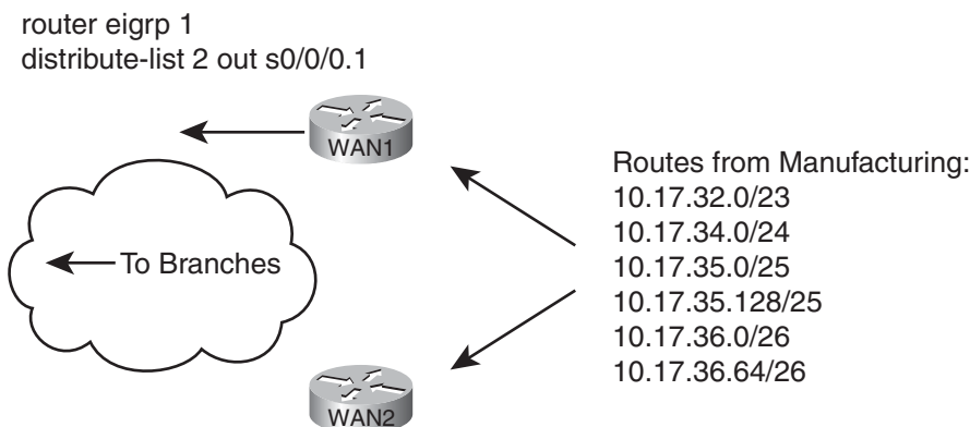
Figure 4-2 Specific Manufacturing Routes to Be Filtered
