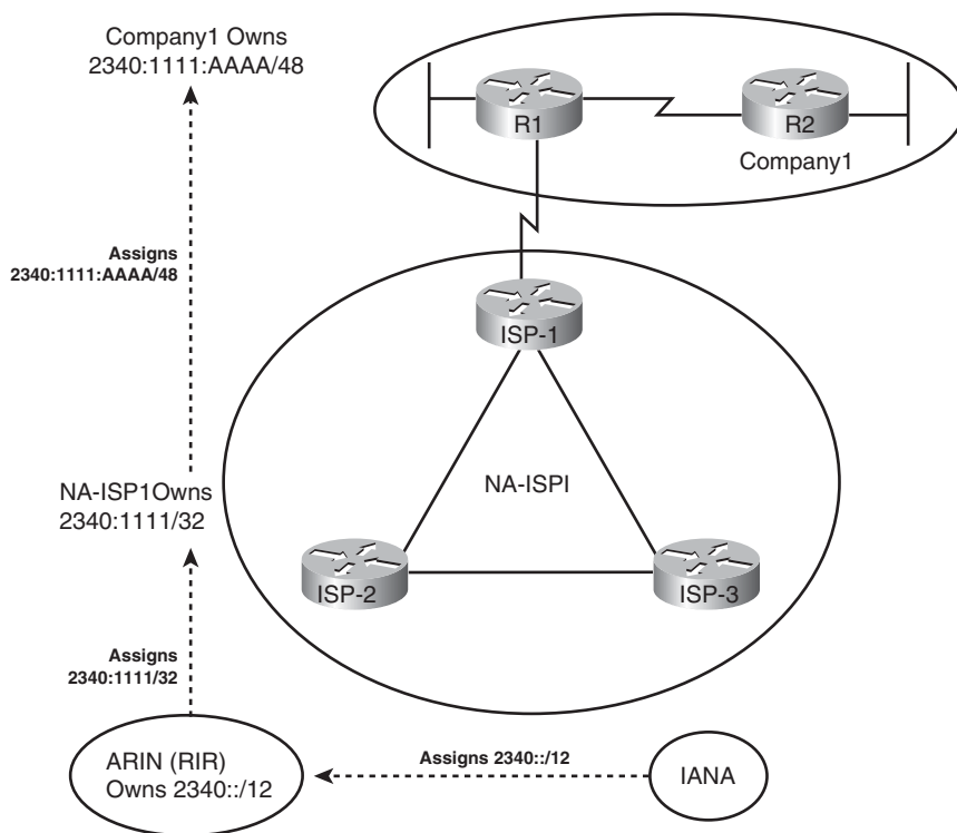
Figure 16-3 Example IPv6 Prefix Assignment in the Internet
