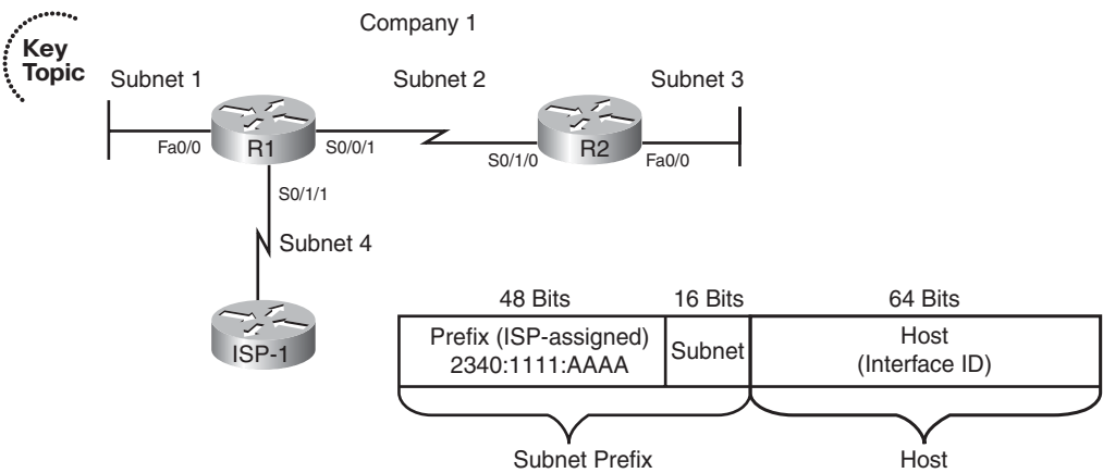
Figure 16-5 Company1—Needs Four Subnets
