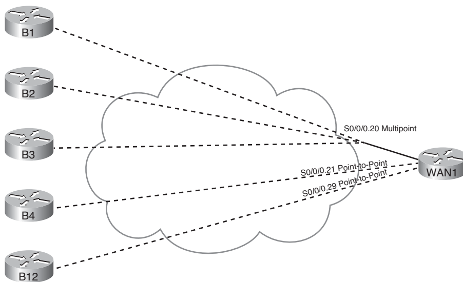
Figure 3-6 One Multipoint and Nine Point-to-Point Subinterfaces
