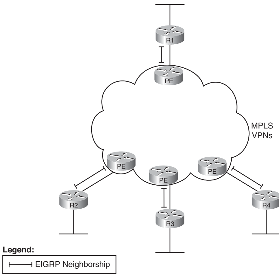
Figure 2-9 EIGRP Neighborhoods over MPLS VPN
